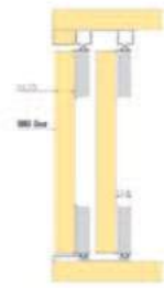
Overlap Version Thickness of door: 16-20mm
